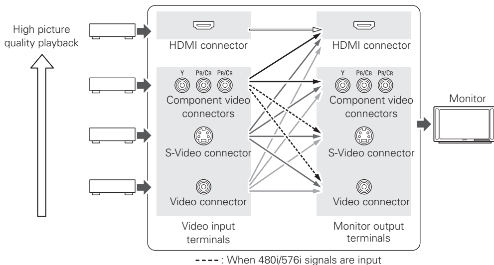
[Flow of video signals inside the AVR-1909]
